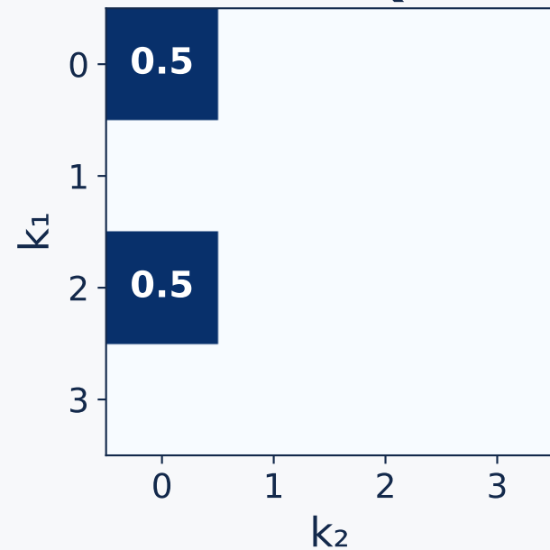
Exact QFT
