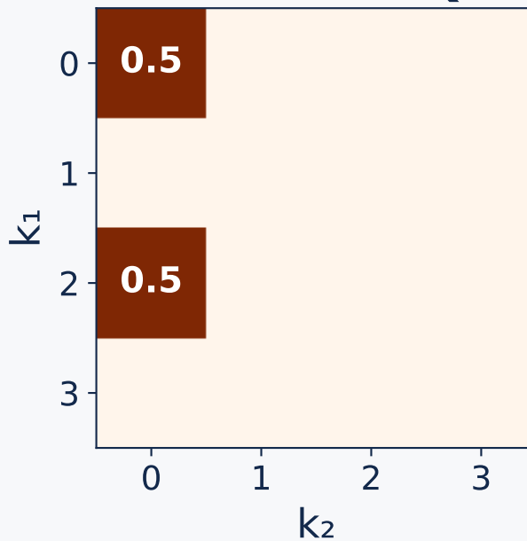
Truncated QFT
